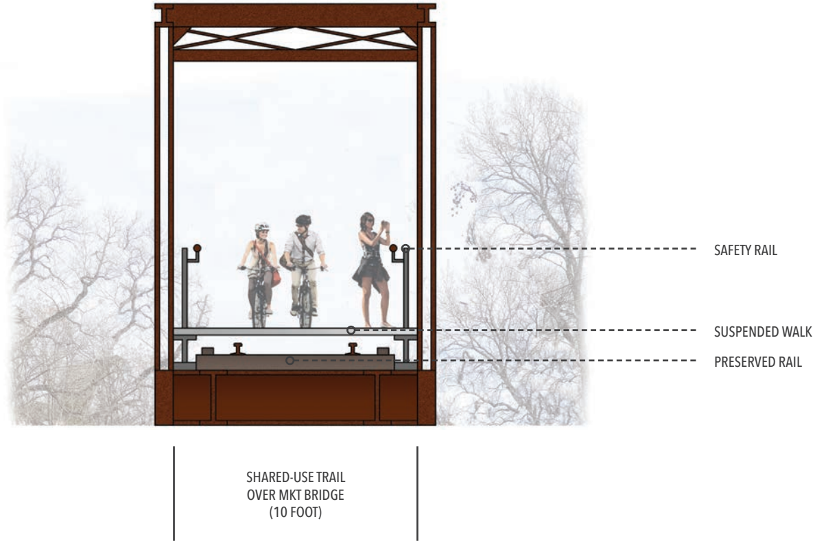
SAFETY RAIL
